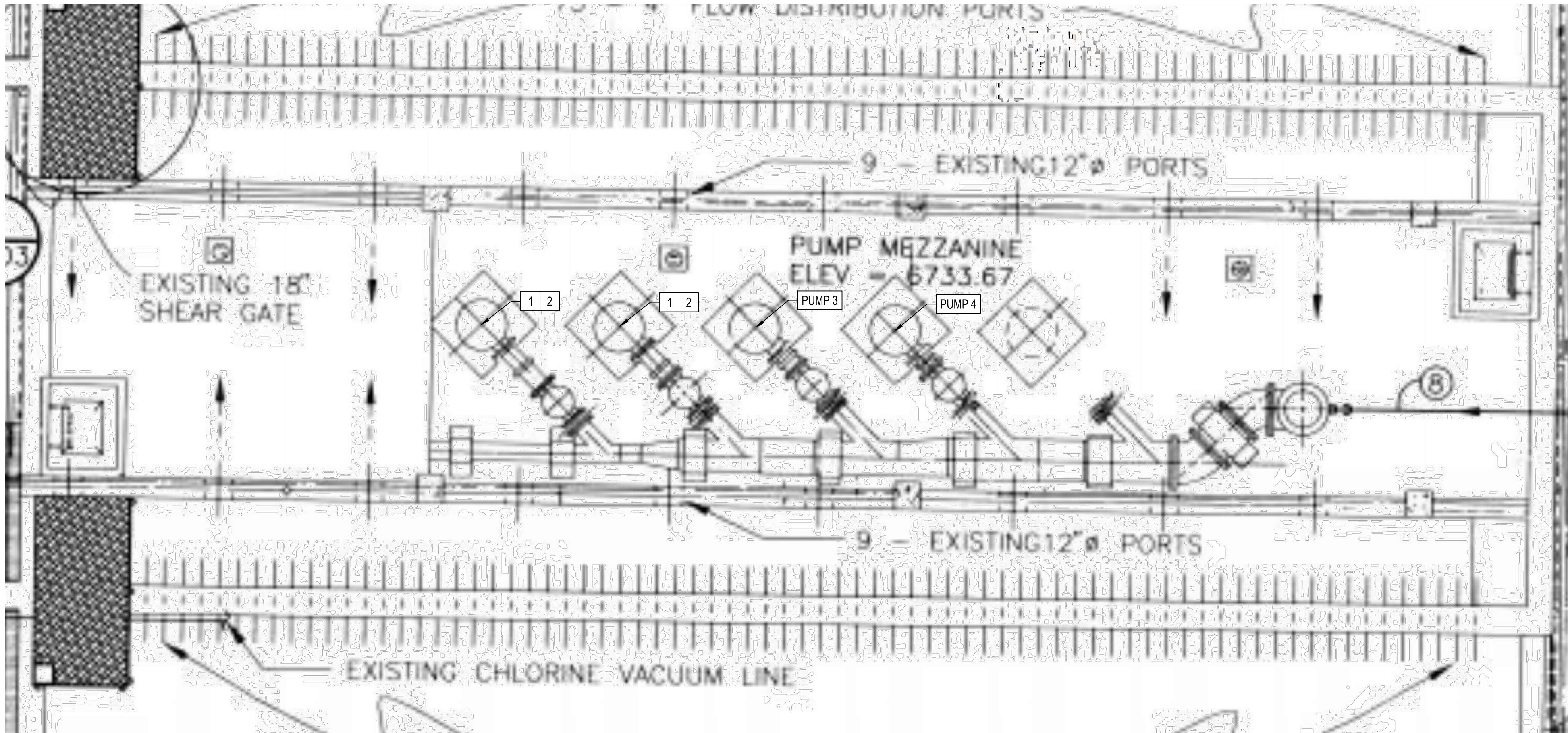
4 EXISTING CLEARWELL BUILDING PLAN SCALE: NOT TO SCALE
